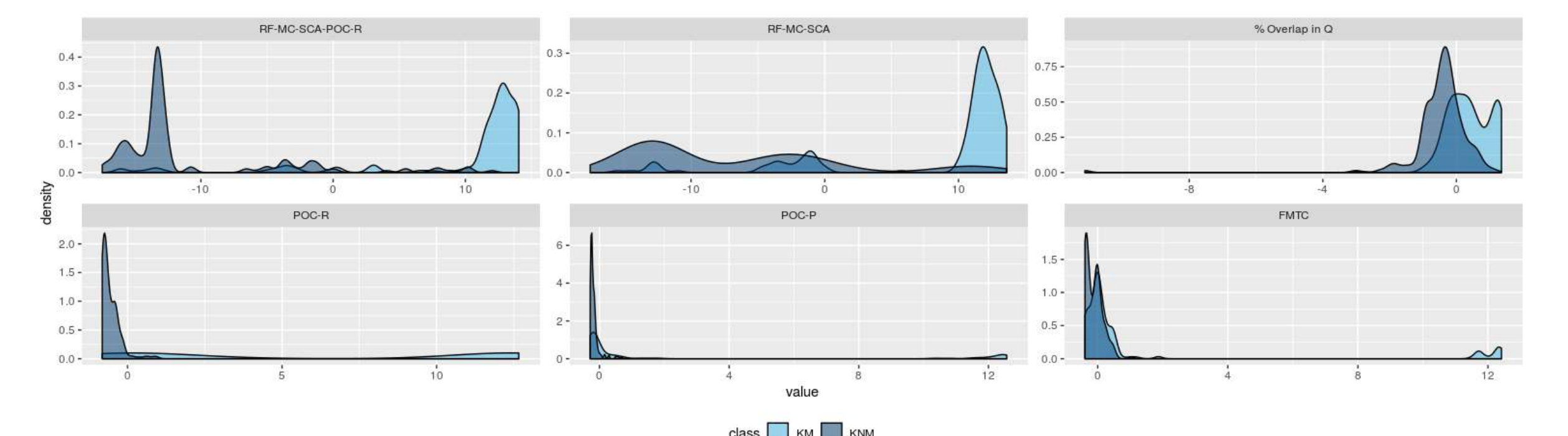
The density of score based likelihood ratio (SLR) in test comparisons is calculated by the training scores. The density of training score in KM and KNM is estimated by kernel density estimation.
