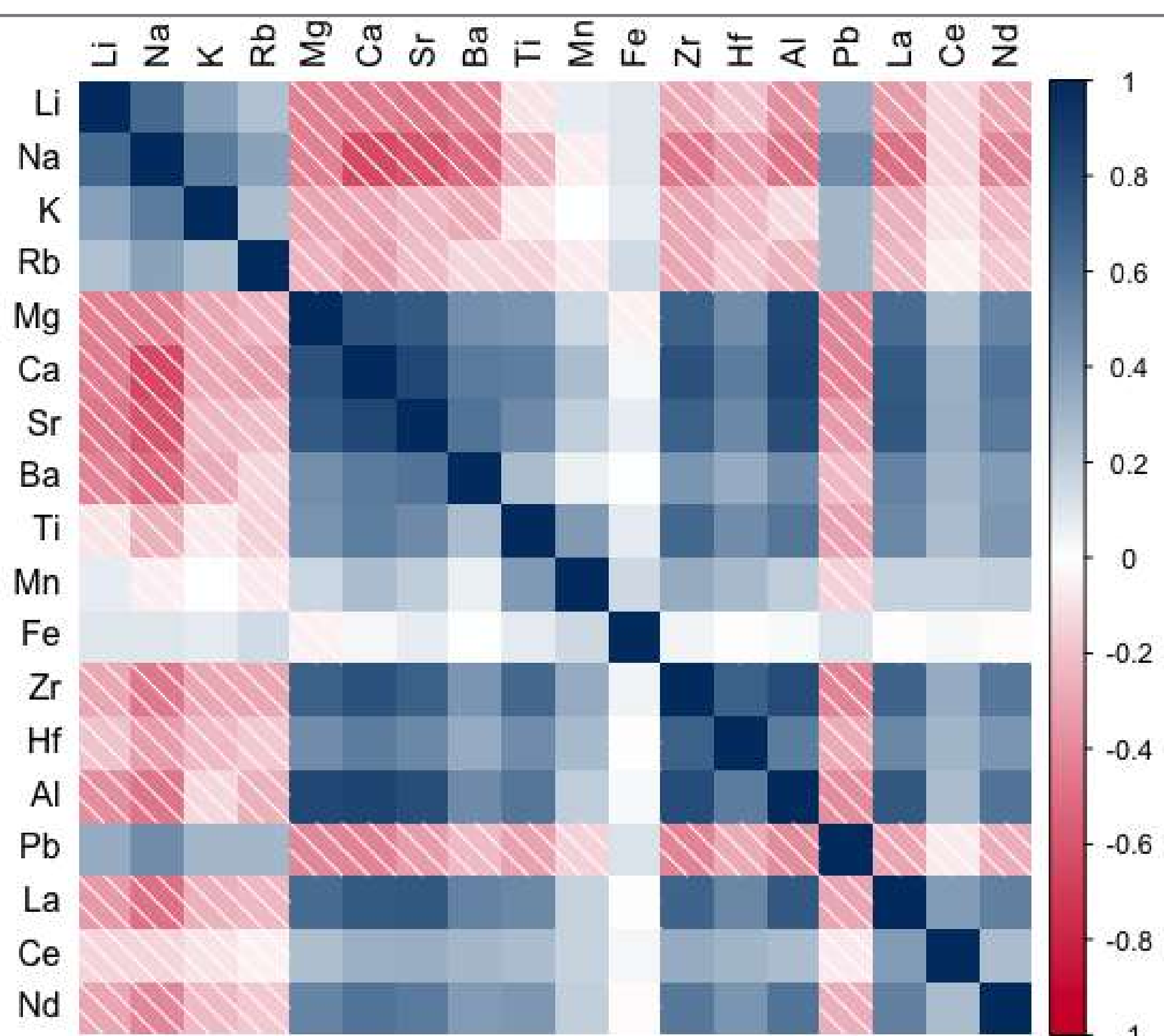
Figure 3: Correlations between elements in glass from Mfr B. Axes ordered according to metal type & mass. We see clear groupings of highly correlated elements, suggesting not all are necessary for source conclusions.
