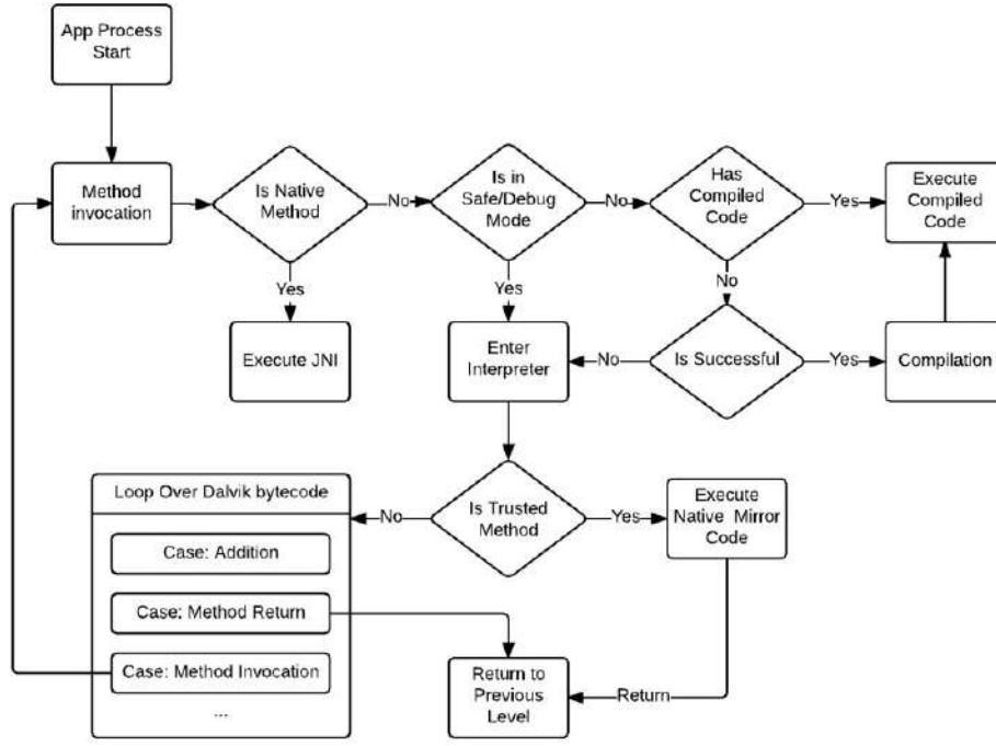
Fig. 2: A Simplified Android ART procedure
