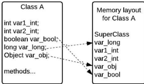
Fig. 4: Memory layout for Class A
