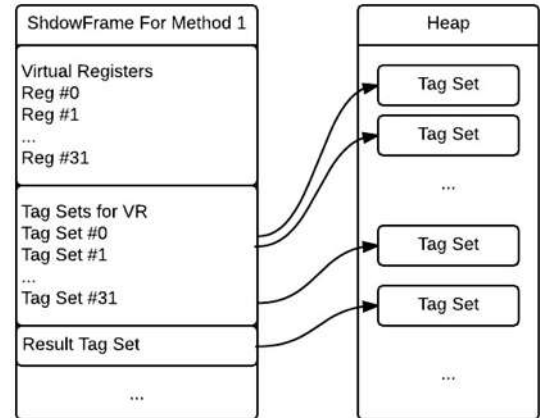
Fig. 3: Taint Storage on App's Stack and Heap Space
