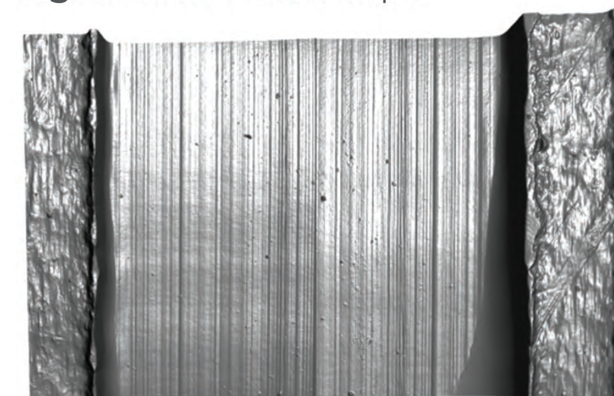
Figure 4: 3D Toolmark scan in lead
