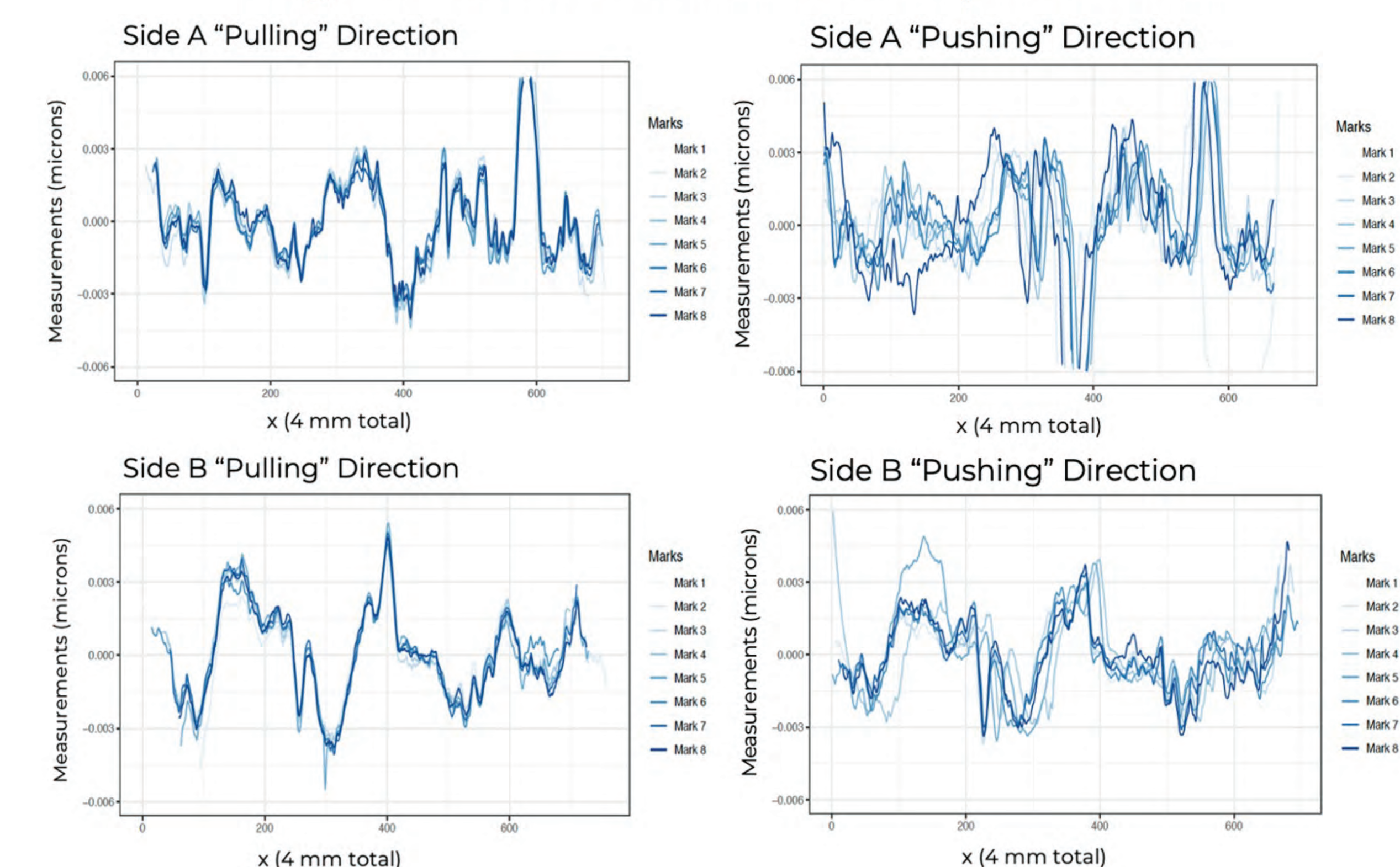
Figure 6: Direction comparison of superimposed marks from small screwdriver 1 side A going in the “pulling” direction (top left) and “pushing” direction (top right) compared to marks from side B going in the “pulling” direction (bottom left) and “pushing” direction (bottom right).
