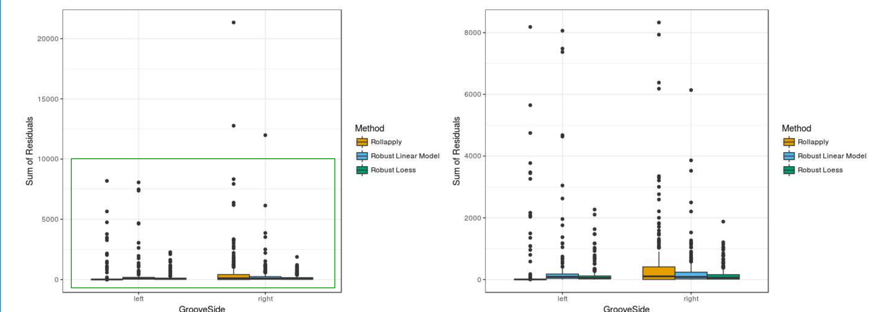
Figure 6. Comparative boxplots of accuracy scores using (1) current method, (2) robust linear models, and (3) robust LOESS. These represent the distribution of accuracy scores over all 208 used lands (left) in the Hamby Barrel Set 44 3D scans, and a zoomed version removing some outlying lands (right). Within each plot, they are split between left groove and right groove.
