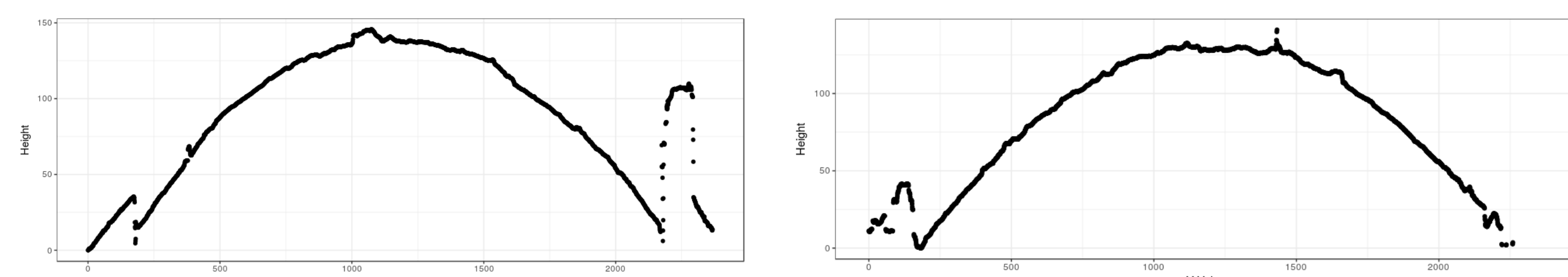
Figure 2. Two examples of bullet land profiles from the Hamby Barrel Set 44 3D scans.
