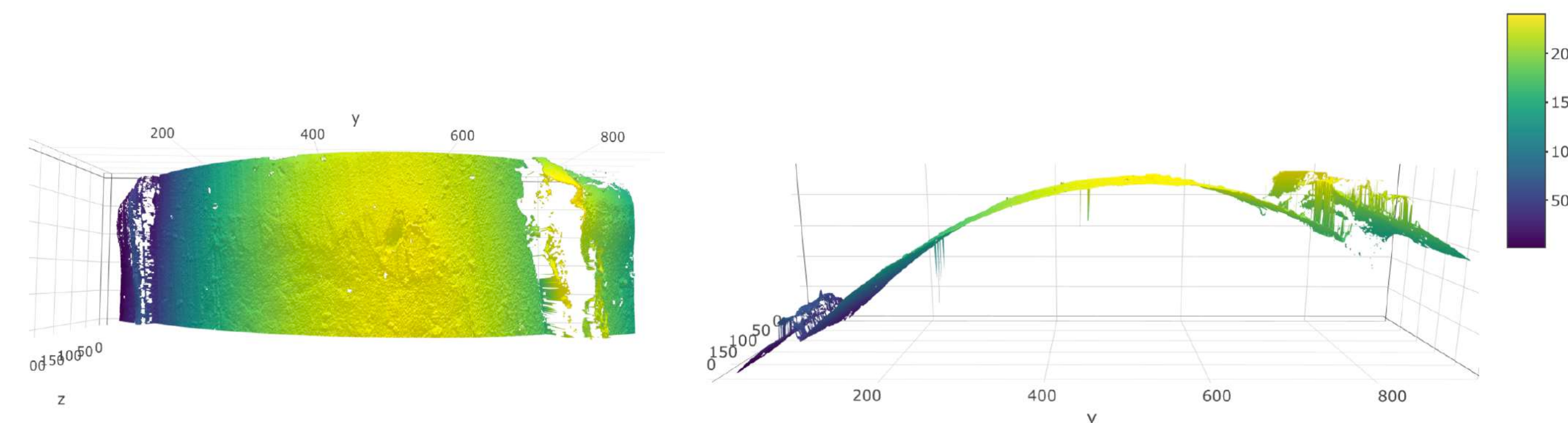
Figure 1. Two views of a high-resolution 3D scan of a single bullet land. When viewing the scan from above (left), striations can be seen along the surface of the land. When viewed from the side (right), the global curved structure of the bullet land can be seen.
