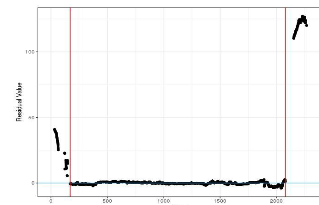
Figure 5. Residuals from a robust LOESS fit overlaid with predicted groove locations.
