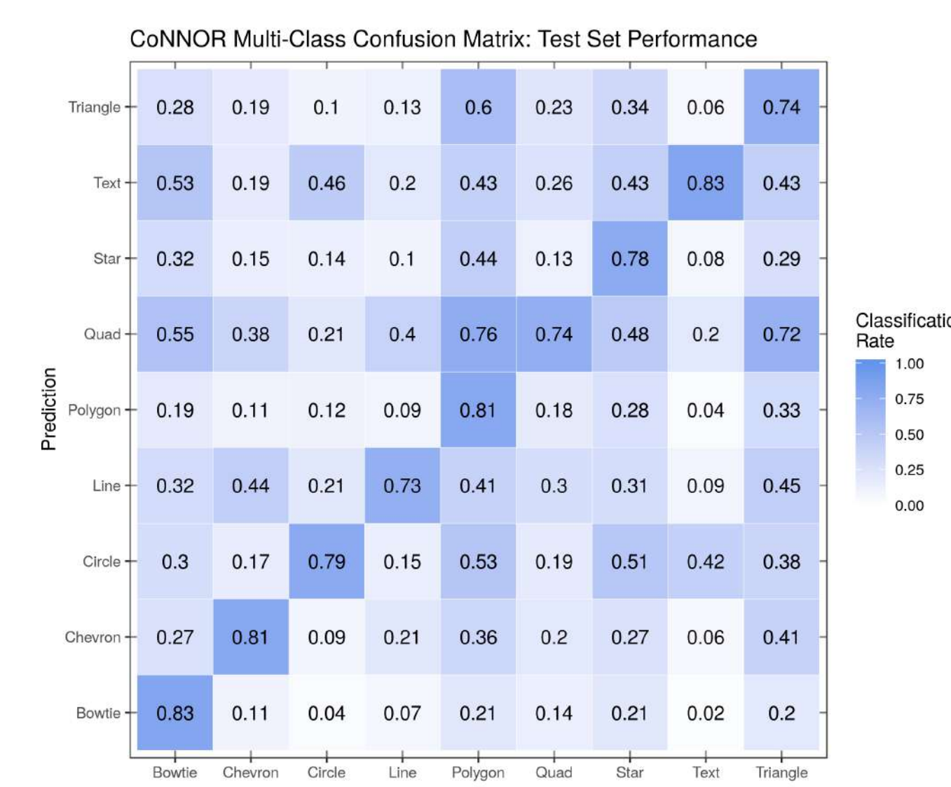
Figure 5: Percent of test images identified as containing a class with probability \geq equal error rate, after accounting for multiple labels
