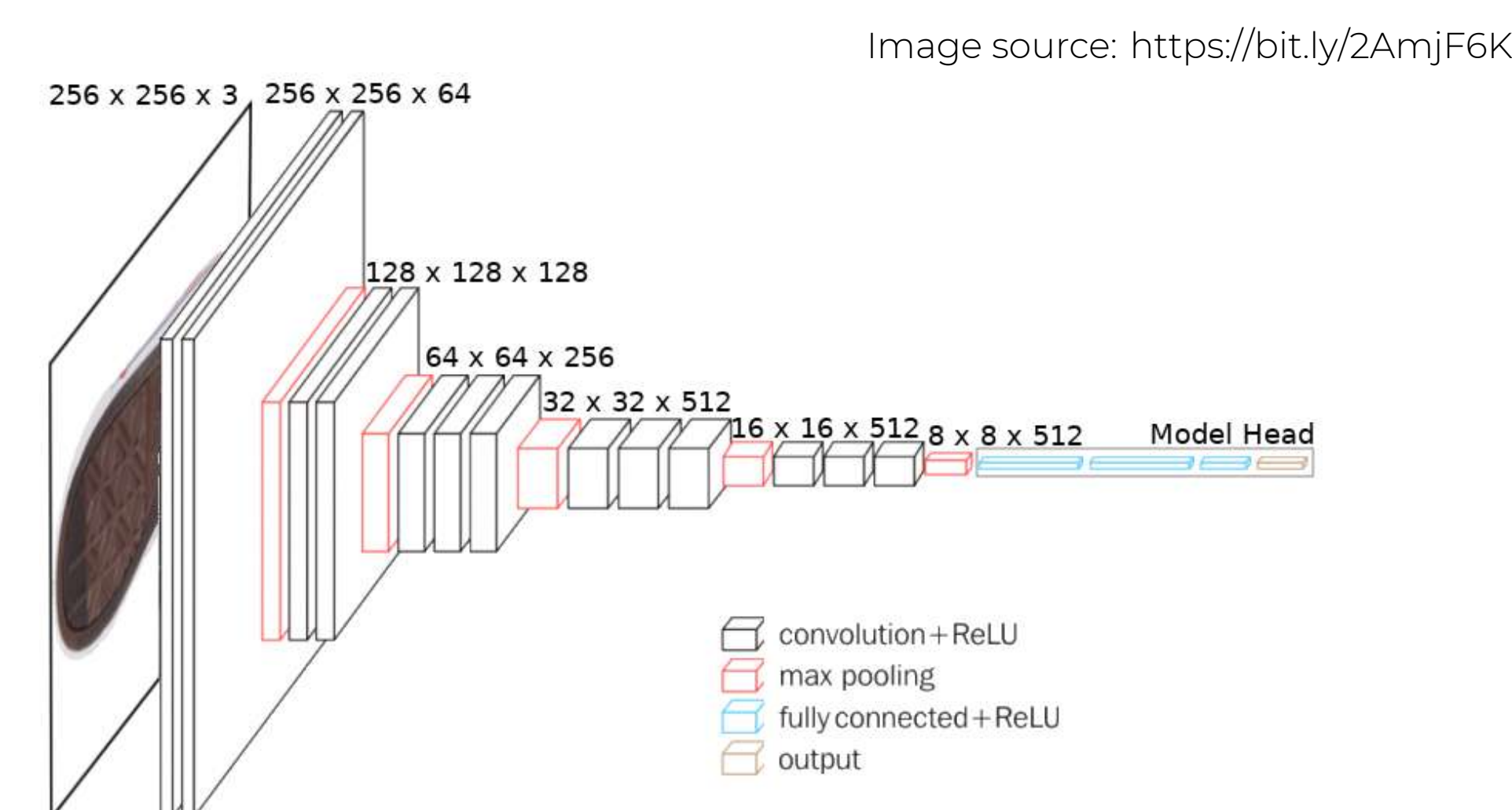
Figure 1: Architecture of VGG16
