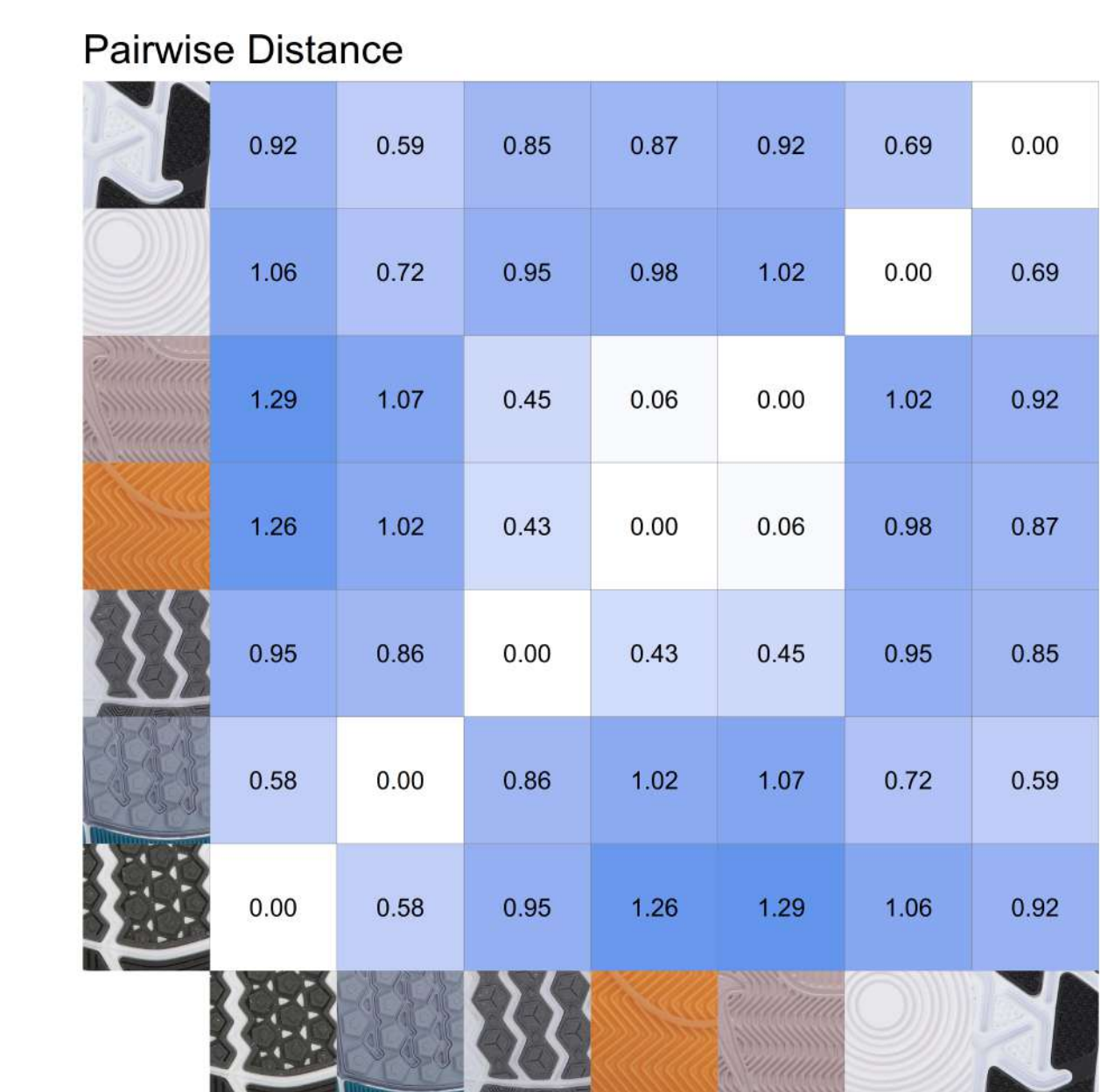
Figure 7: Pairwise Euclidean Distance between selected example images
