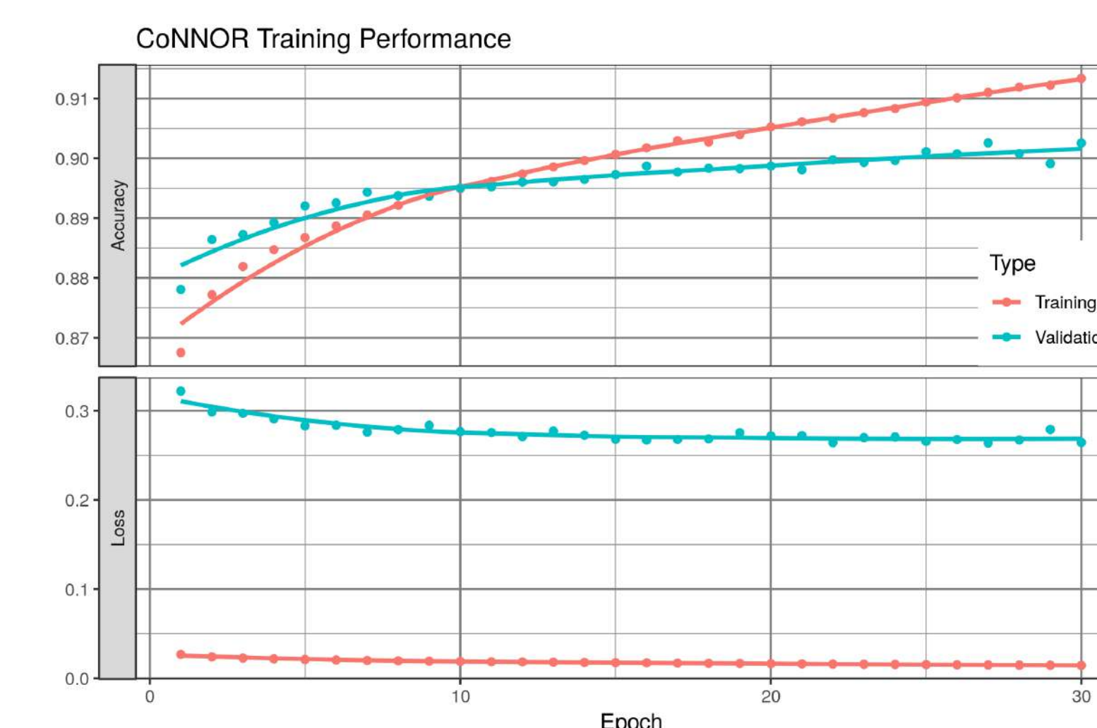
Figure 4: Training and Validation accuracy and loss for each epoch of the fitting process.
